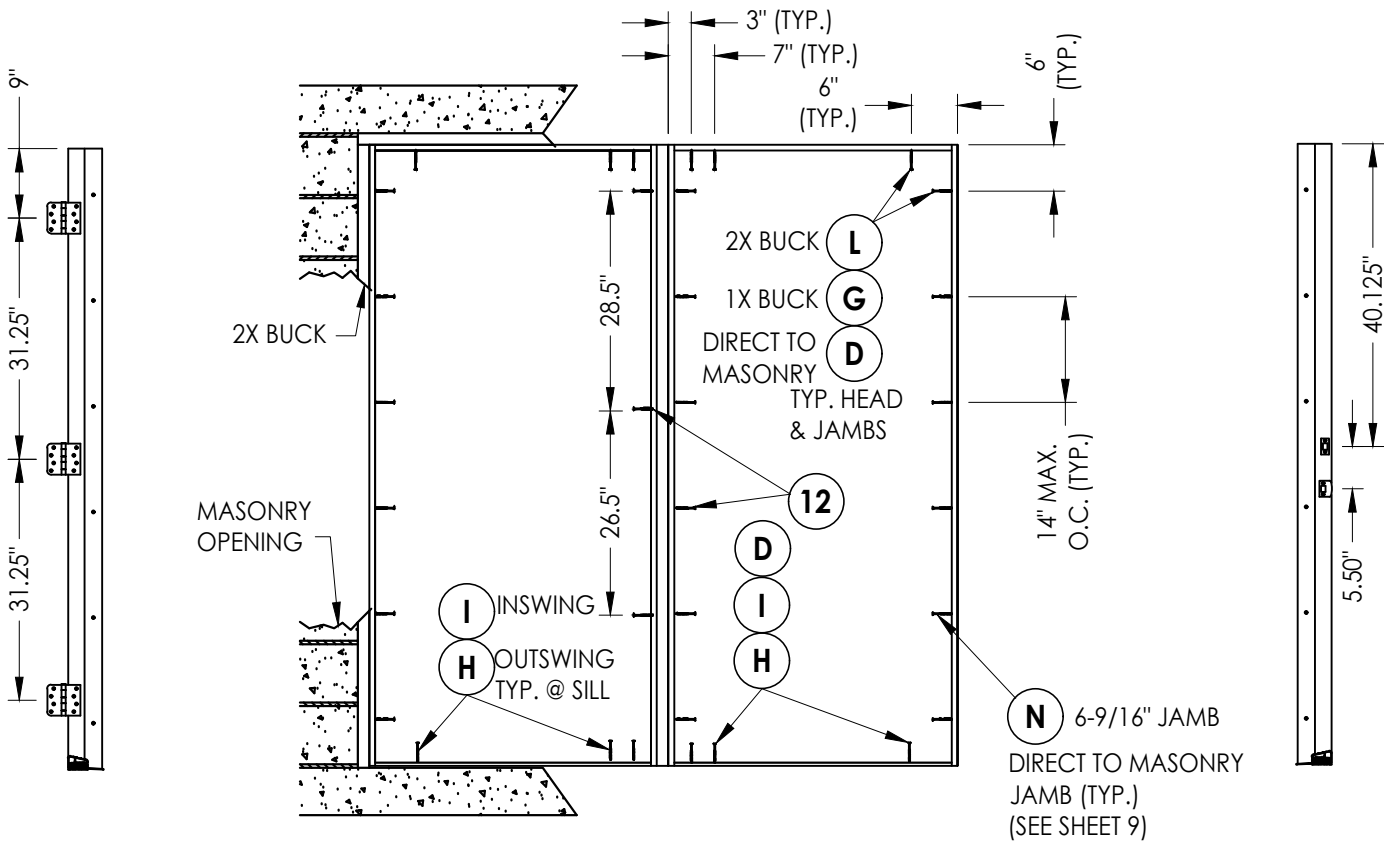
FRAME ANCHORING Masonry 2X buck construction
