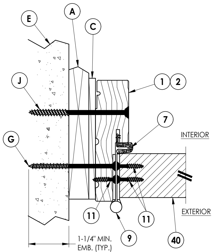
1 HORIZONTAL CROSS SECTION 6 Shown w/ 1X sub-buck Outswing shown (Inswing similar)
