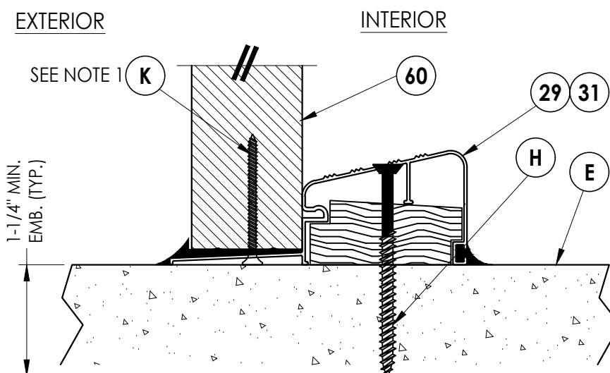
4 VERTICAL CROSS SECTION 8 Outswing configuration
