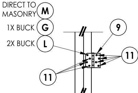
HINGE DETAIL
